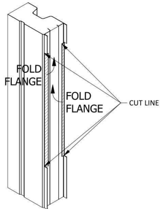
SNIP DETAIL A
