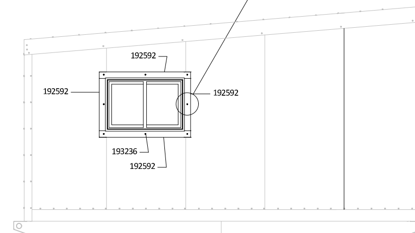
OUTSIDE TRIM VIEW(X2)
