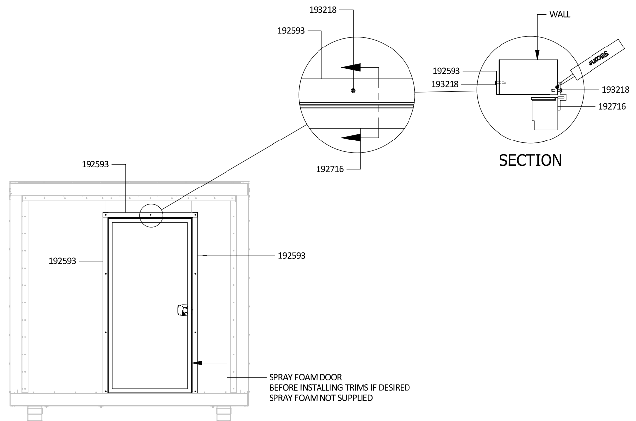
(INSIDE TRIM VIEW)
